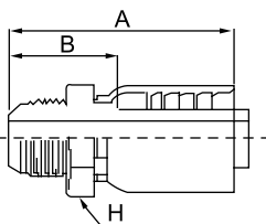
MJ JIC 37° Male Rigid Straight
