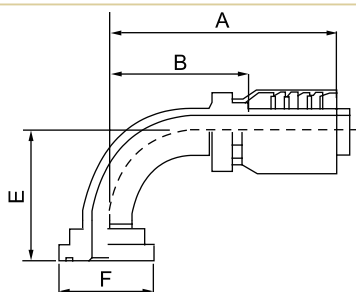
PA SAE Flange 90° Elbow Standard Type
