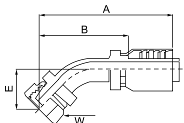
NML DIN 20 078 A Light Series Metric Female Swivel 45° Elbow
