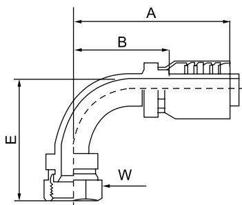
NJ JIC 37° Female Swivel 90° Elbow
