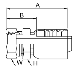
NPB BSP Female Flat Face Swivel Straight
