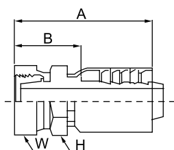
NML DIN 20 078 A Light Series Metric Female Swivel Straight
