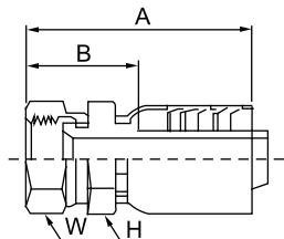
NJ JIC 37° Female Swivel Straight
