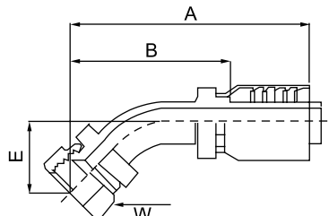
NJ JIC 37° Female Swivel 45° Elbow
