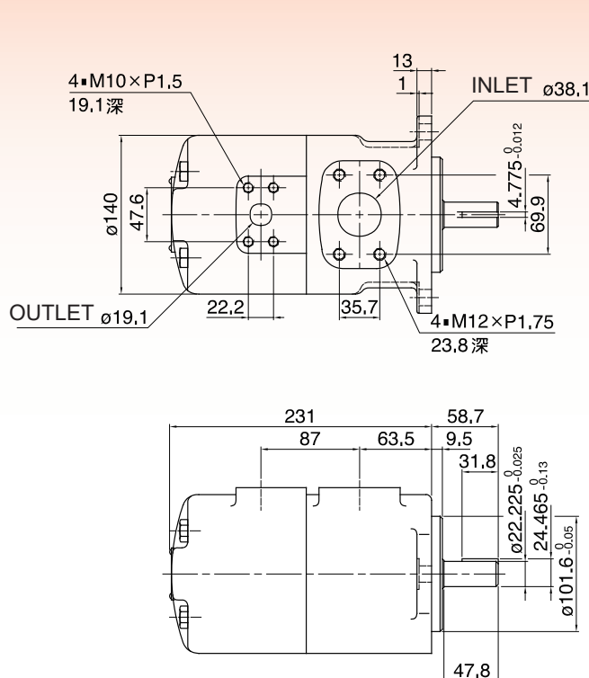
IVPQ1 Flange Mounting (Shaft Model No.1)
