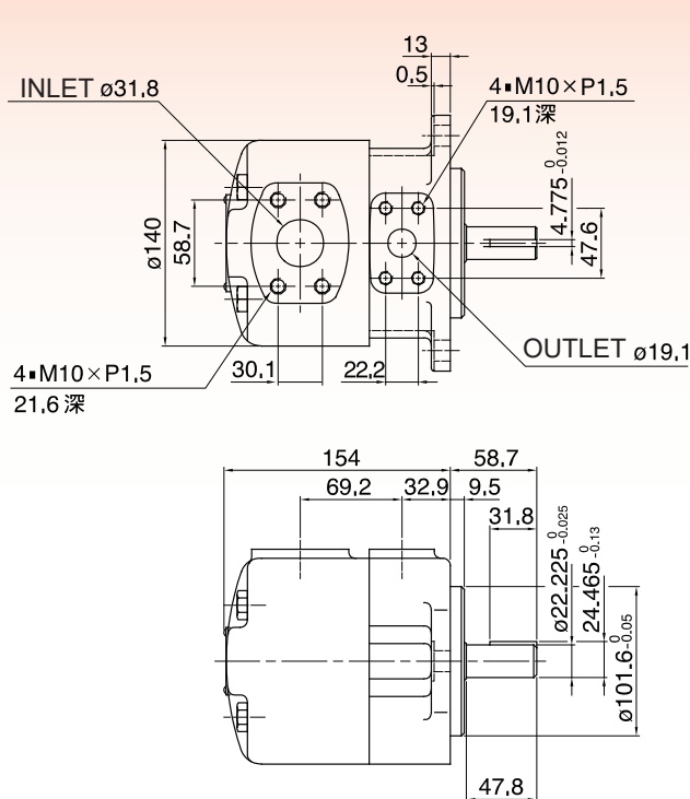
IVP1 Flange Mounting (Shaft Model No.1)
