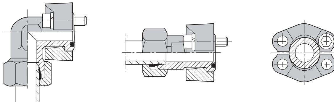
ELBOW SAE-FLANGE CONNECTION WFS
