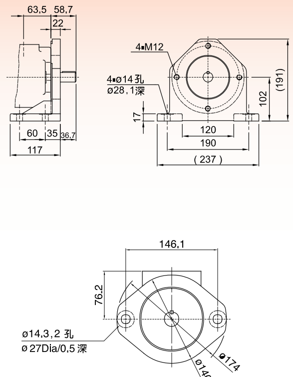
IVPQ1 Flange Mounting (Shaft Model No.1)
