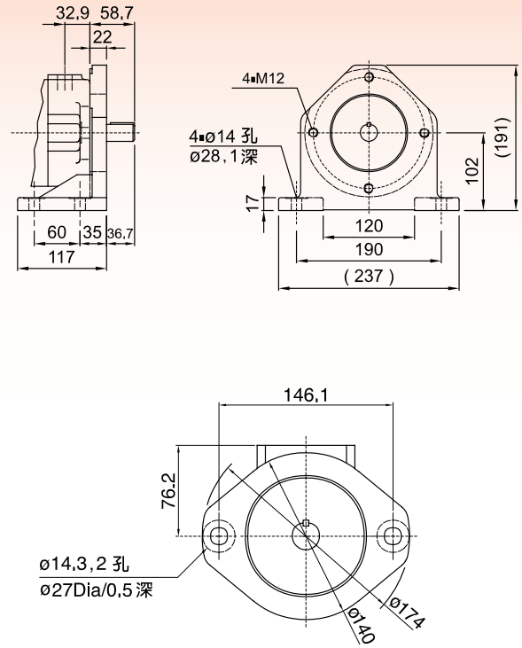
IVP1 Foot Mounting (Shaft Model No.1)
